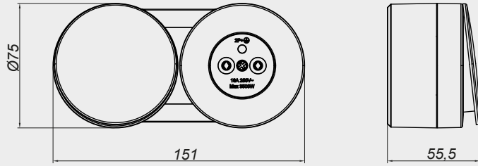
ANAHTAR B.D. + UPS PRİZ
