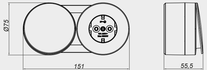
ANAHTAR B.D. + TOPRAKLI PRİZ
