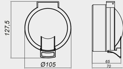
W.P. TOPRAKLI PRİZ
