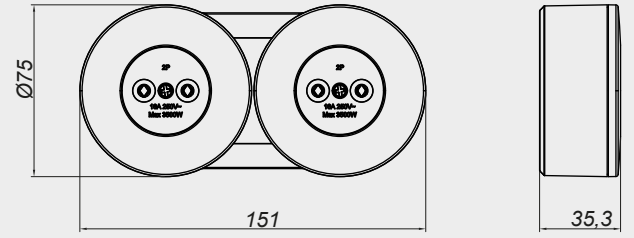
PRİZ + PRİZ
