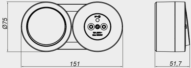
ANAHTAR + UPS PRİZ
