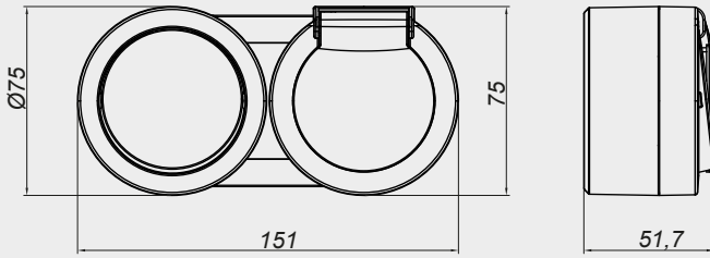
ANAHTAR + KAPAKLI TOPRAKLI PRİZ
