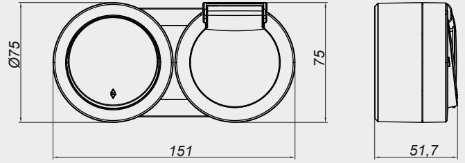
VEAVİEN + KAPAKLI TOPRAKLI PRİZ
