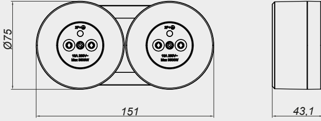
UPS PRİZ + UPS PRİZ
